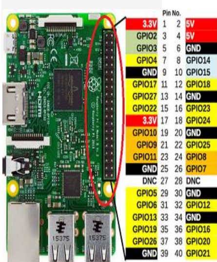
Gambar 2. 2 Raspberry Pi[2]
