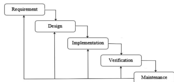
Gambar 1. 1 Metode Waterfall
