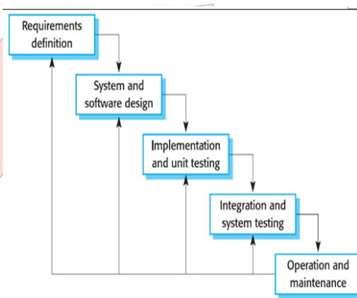
Gambar 1. 1 Waterfall Presman [1]
