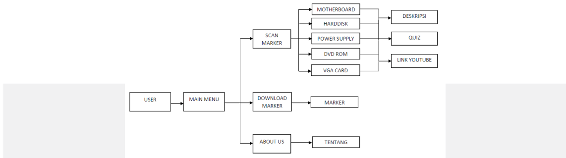
Gambar 3. 6 Usecase Diagram
