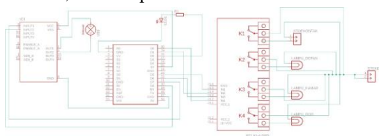
Gambar 4.1 Skematik Hardware
