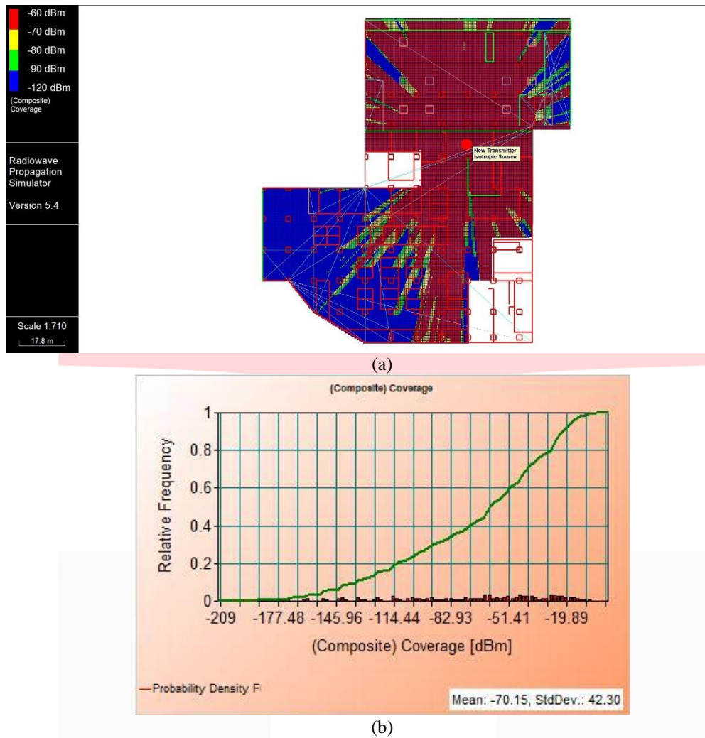
Gambar 12 Kondisi coverage plot (a) dan grafik histogram (b) area boarding lounge lantai 3
