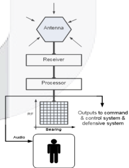
Gambar 2.2 ESM (Electronic Support Measure)
