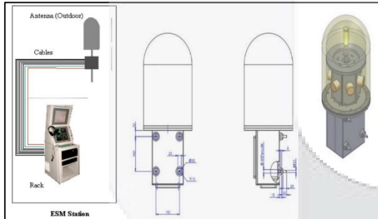
Gambar 2.1 (a) ESM Station [5] (b) Antena Outdoor ESM [5]
