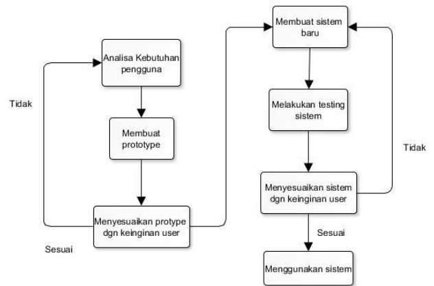
GAMBAR 1. 1 METODE PROTOTYPE [2]
