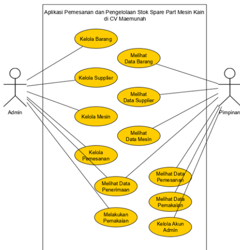
Gambar 2-2 Use case
