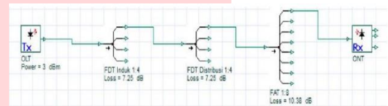
Gambar 13 Splitter 4-4-8
