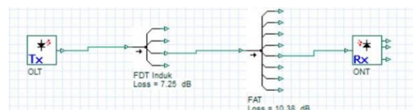
Gambar 11 splitter 4-8
