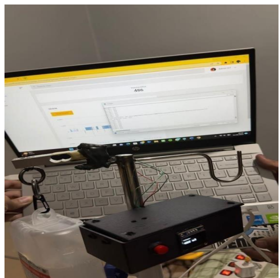
Gambar 4. Tampilan Mesin Sistem Monitoring Infus
