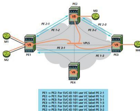
Gambar 2.5 PW Signaling [3]
