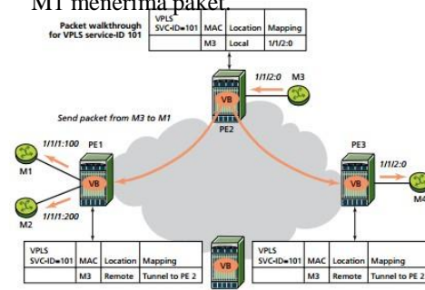
Gambar 2.6 VPLS Learning [3]
