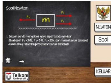
Gambar 3.12 Soal Newton
