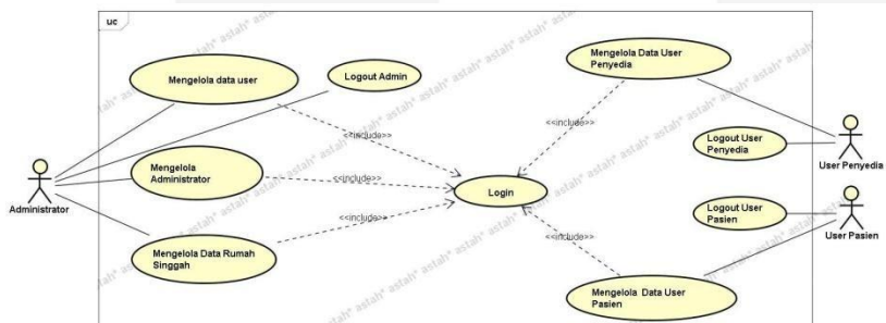
Gambar 5 Diagram Usecase
