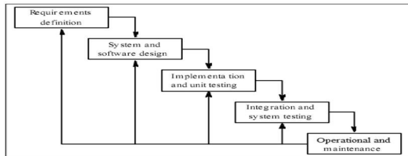
Gambar 1-1 Metode Waterfall
