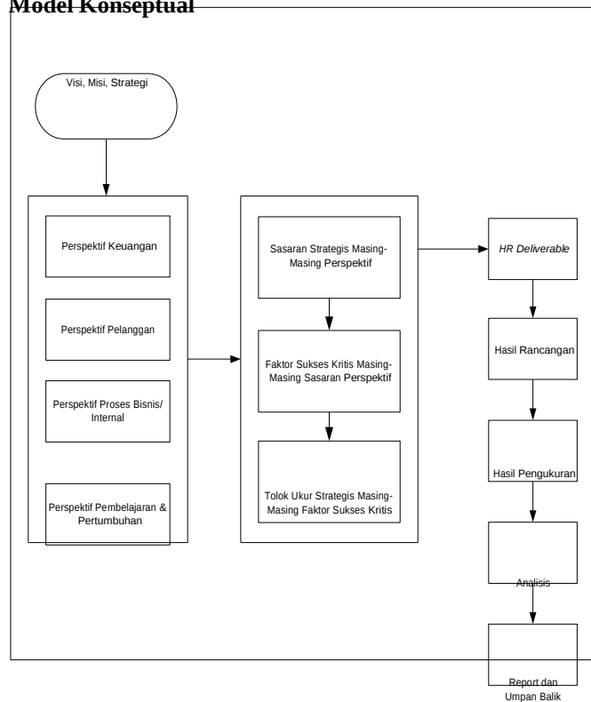
Gambar 2. Model Konseptual
