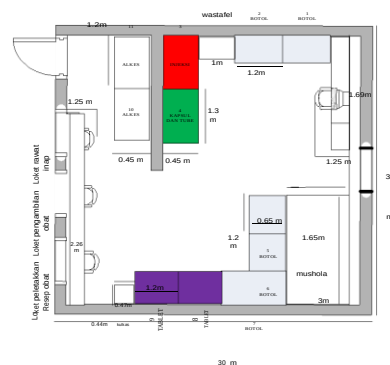
Gambar 9 Layout Improvement Apotek
