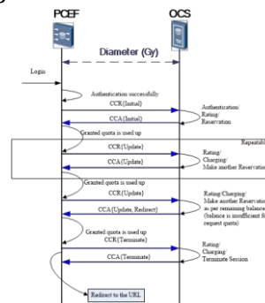
Gambar 3.4 Flow Diagram Proses Charging di PCEF dan OCS
