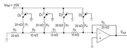
Gambar 3 Rangkaian-Dasar-R2R-Ladder-DAC [12]
