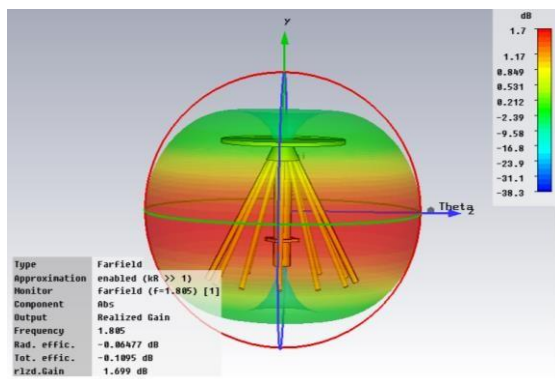
Gambar 9. Hasil Simulasi 3D Polaradiasi Azimuth
