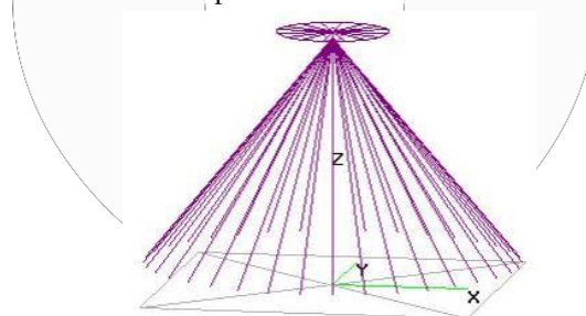
Gambar 1. Antena Discone Wire
