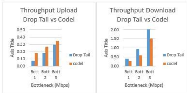
Gambar 4-7 Perbandingan Throughput Drop Tail vs Codel
