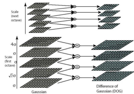
Gambar 2.2 Representasi Difference-of-Gaussian[7]
