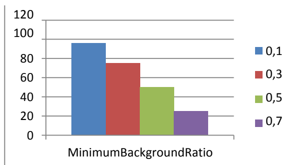
Gambar 4-4 Grafik MinimumBackgroundRatio
