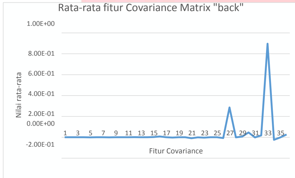
Gambar 3.3 Rata-rata fitur covariance matrix “Back”
