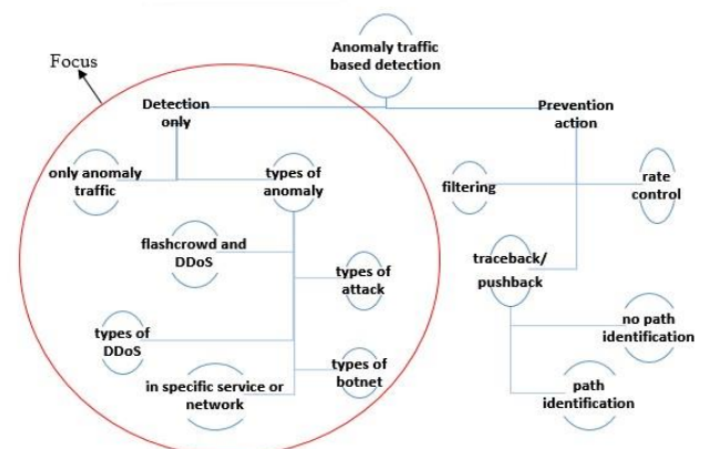
Gambar 1 Capability focus taxonomy [3]
