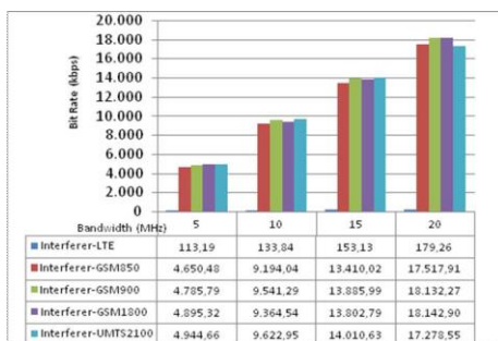
Figure 4.3 Throughput for frequency 2100MHz
