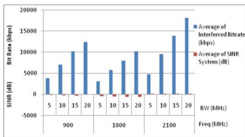
Figure 6.3 LTE interfered GSM900
