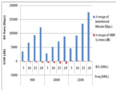
Figure 6.2 LTE interfered GSM850
