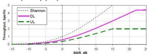
Figure 3.2 Throughput vs SNIR for Baseline E-UTRA Coexistence Studies [3]
