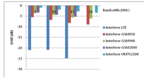
Figure 5.2 SINR for frequency 1800MHz
