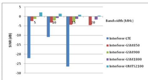
Figure 5.1 SINR for frequency 900MHz
