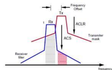
Figure 2.1 Interference as a result of limited ACLR and ACS [3]
