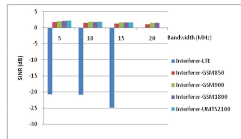
Figure 4.3 SINR for frequency 2100MHz
