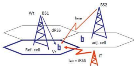
Figure 3.1 Interference mechanism in LTE network
