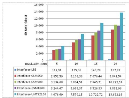
Figure 4.2 Throughput for frequency 1800MHz
