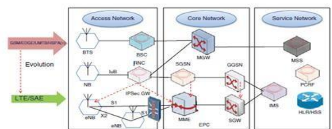
Figure 1.1 Evolution from 2G/3G/HSPA(+) to LTE [1]
