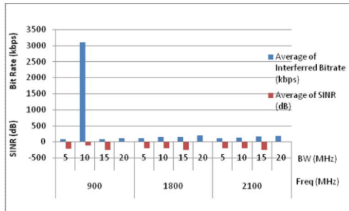
Figure 6.1 LTE interfered by LTE; Throughput vs SINR
