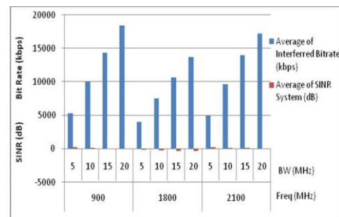
Figure 6.5 LTE interfered UMTS2100
