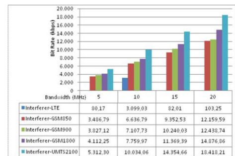
Figure 4.1 Throughput for frequency 900MHz
