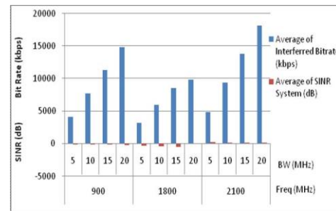
Figure 6.4 LTE interfered GSM1800
