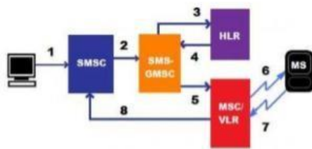
Gambar 2.2 Diagram alir SMS [1]
