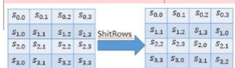
Gambar 2.4.4 Proses ShiftRows [3]
