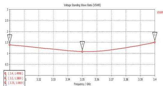
Gambar 3.4 VSWR Antena
