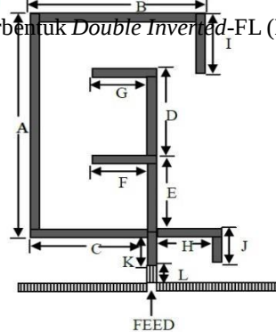
Gambar 2.3 Antena Double inverted FL [3]
