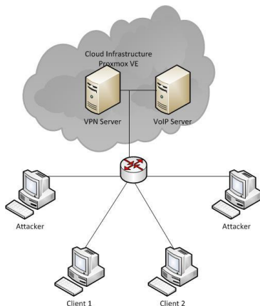
Fig 1. Network Topology
