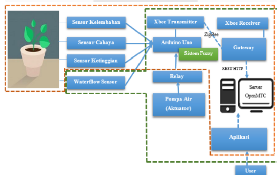
Gambar 4 Skema Sistem Monitoring Tanaman
