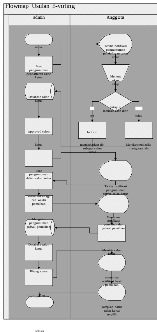
Gambar 3-2 Flowmap Sistem Usulan e-voting
