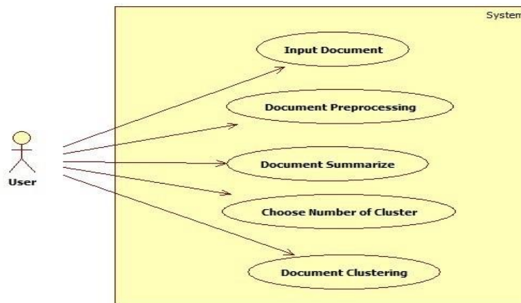
Gambar 2.2 Use Case Diagram sistem
