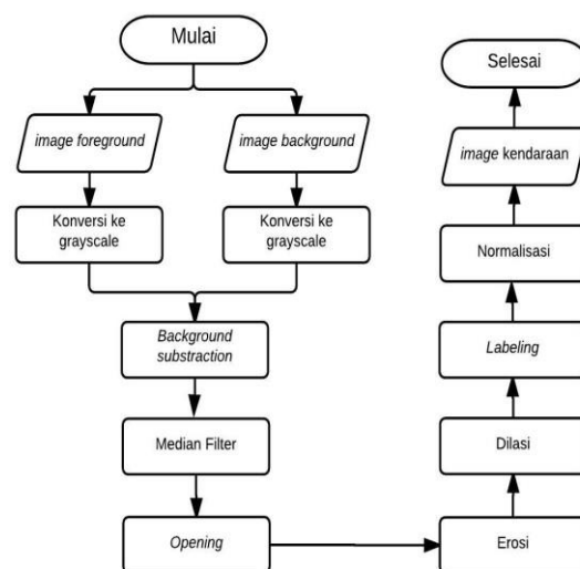
Gambar 4 Flowchart Preprocessing
