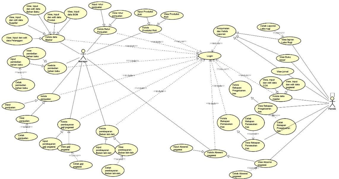
lampiran 1 Usecase Diagram
