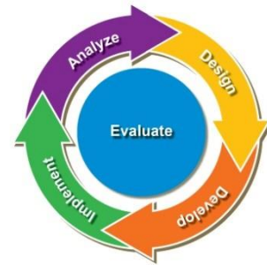
Gambar 1 Metode ADDIE [9]
