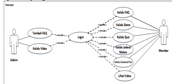
Gambar 2 Usecase Diagram
