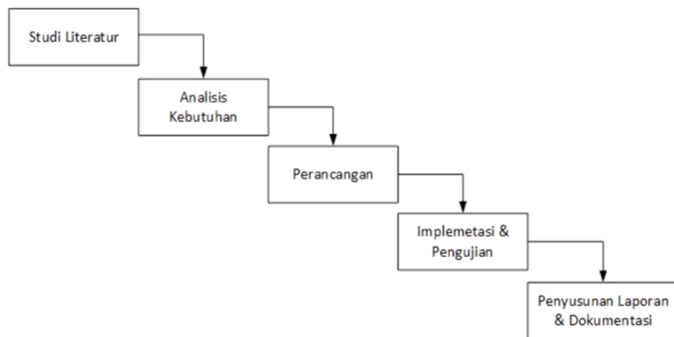
Gambar 1-1 Metode Waterfall
