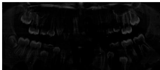
Gambar 3.6 Citra Grayscale
