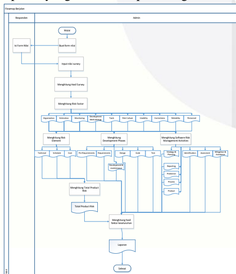
Gambar 3-1 Flowmap berjalan
