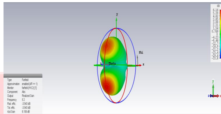
Gambar3.7 Gain Antena 4 Elemen Azimuth
