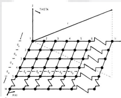
Gambar 1.2 Geometri Planar Array [7]
