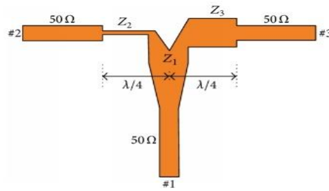
Gambar 1.3 T-Junction 70,7 ohm
