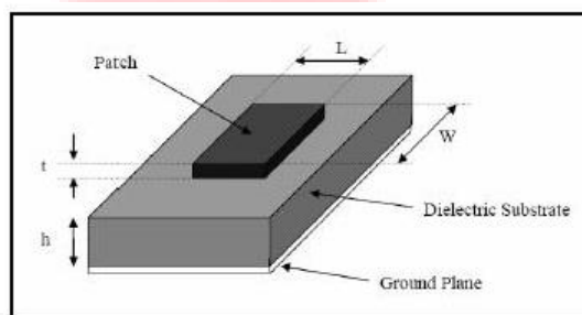
Gambar 1.1 Antena Mikrostrip [5]
