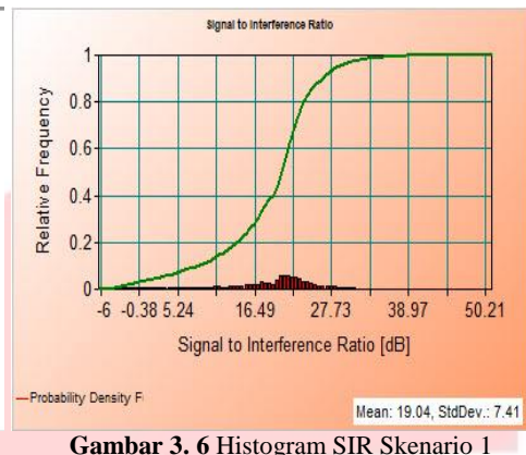
Gambar 3. 6 Histogram SIR Skenario 1
