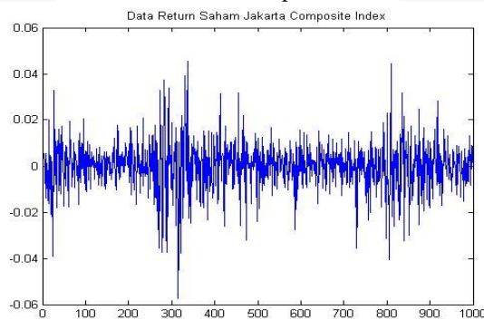
Gambar 3 Data Return Jakarta Composite Index
