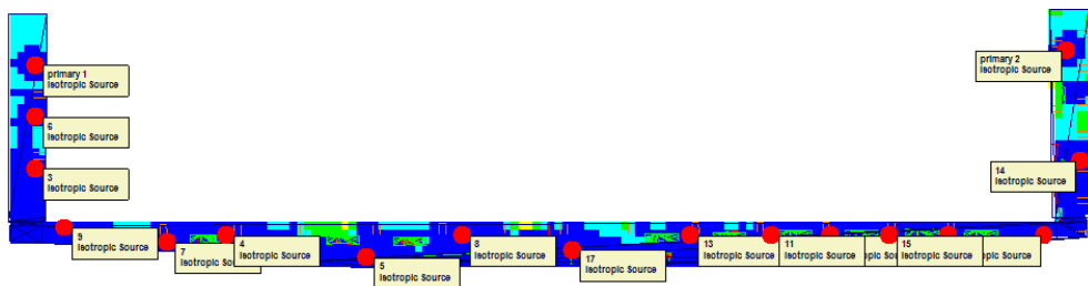
Gambar 3.7 (a) Simulasi SIR Skenario 1 (b) Histogram SIR Skenario 1
