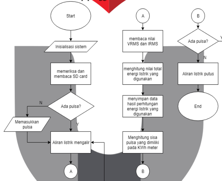
Gambar III- 10. Diagram Alir Sistem
