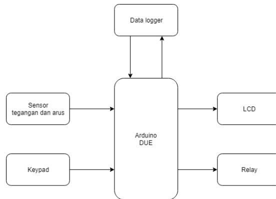
Gambar 3- 2. Diagram blok data
