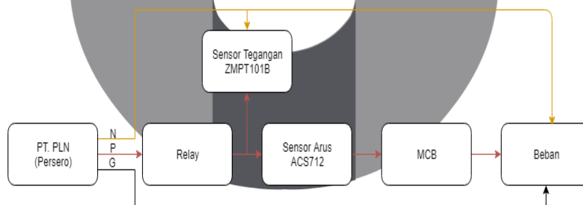
Gambar 3-1. Diagram blok daya
