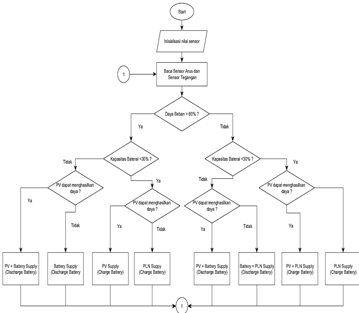
Gambar 4. Flowchart Sistem
