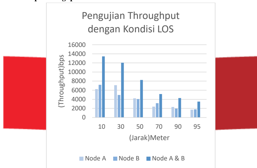
Gambar 6 Grafik Hasil Pengujian Throughput Monitoring
