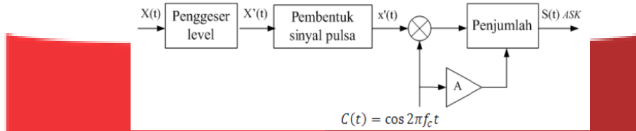
Gambar 2.4 Blok Diagram Modulator ASK
