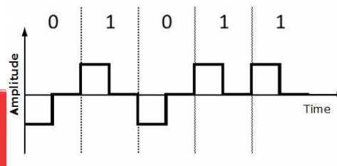
Gambar 2.2 Sinyal Digital
