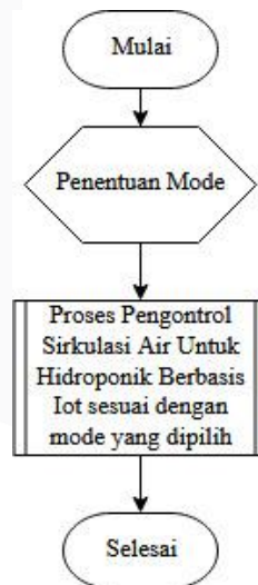
Gambar 3.2 Flowchart Sistem
