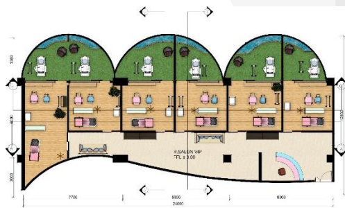
Gambar 7. Layout Salon
