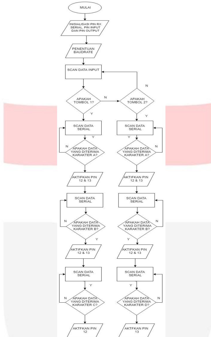
Gambar 3.4 Implementasi Sistem Receiver
